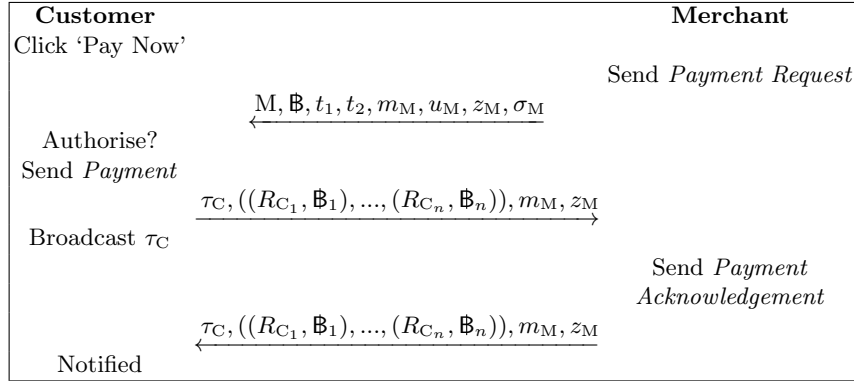
Fig. 3. Message contents for the Payment Protocol
