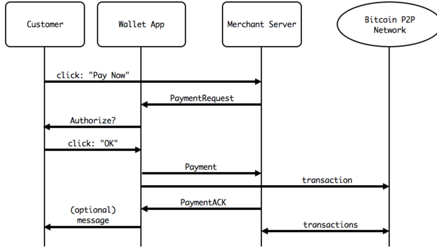
Fig. 2. Overview of the Payment Protocol [4]
